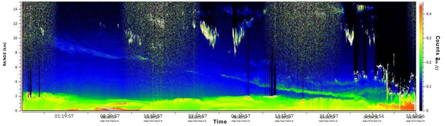
High altitude aerosol descends and merges into local boundary layer over a 3-day period.
