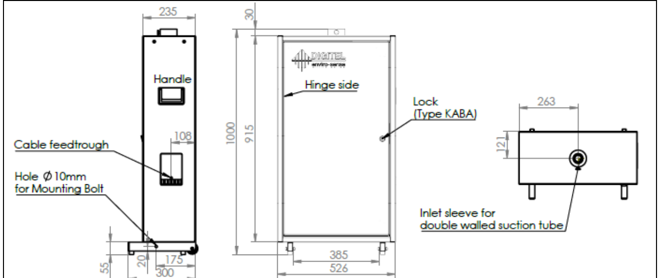
Figure 4: Dimensions of the field housing
