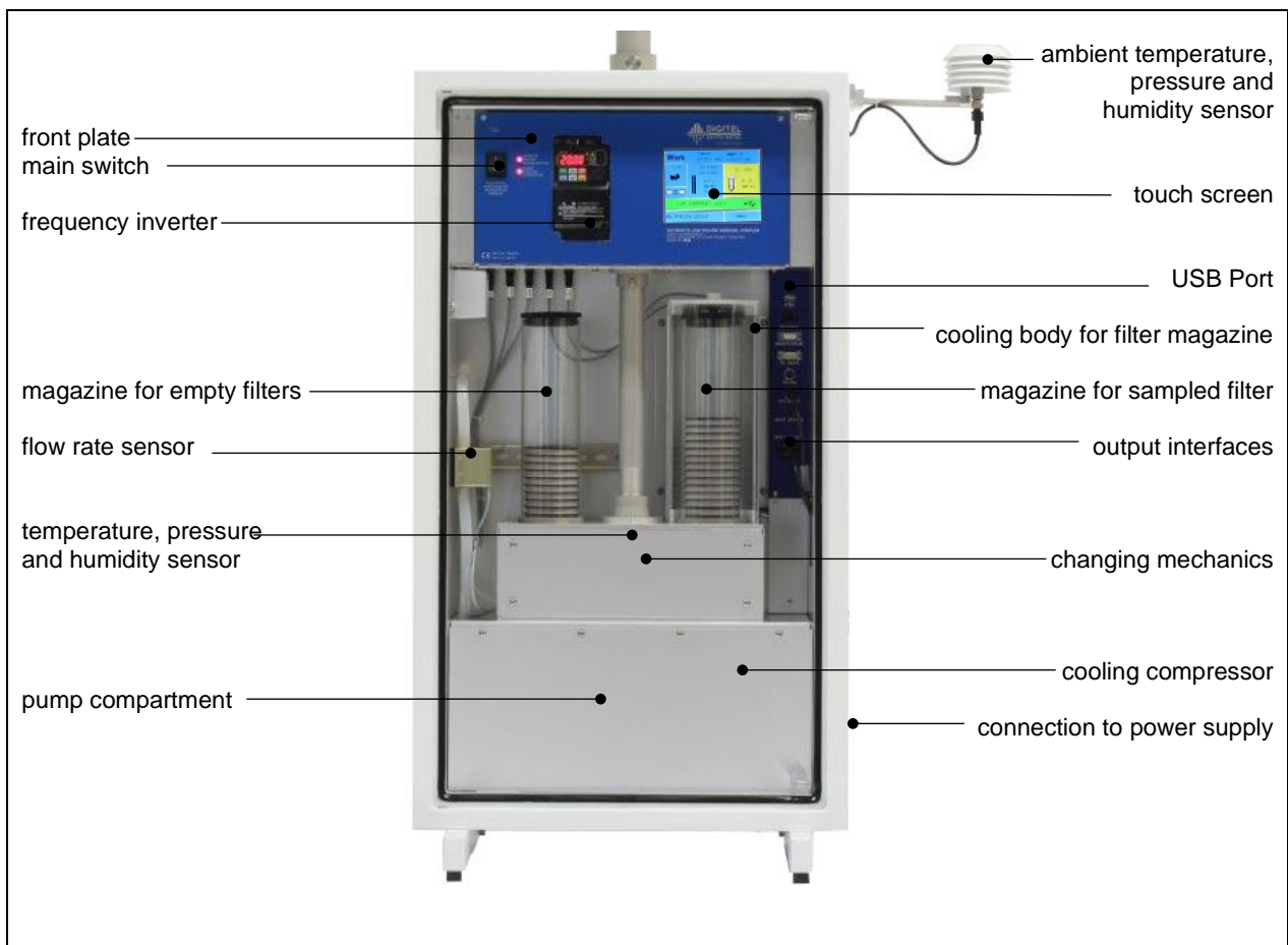
Figure 2: Components
